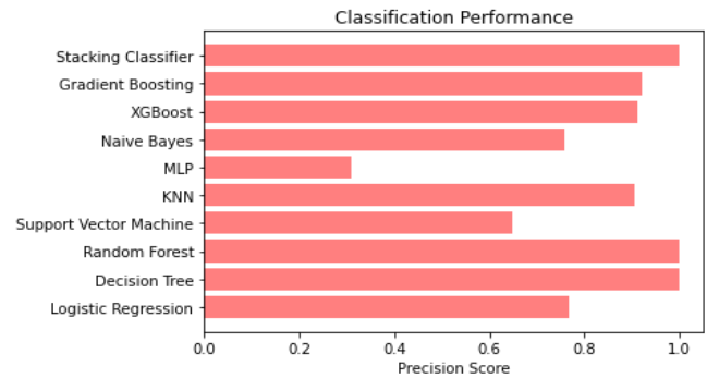
Fig 13 Precision graph
