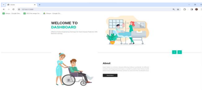
Fig 17 Home page
