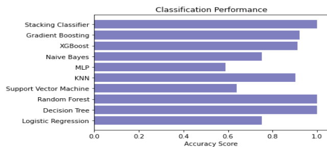
Fig 12 Accuracy graph
