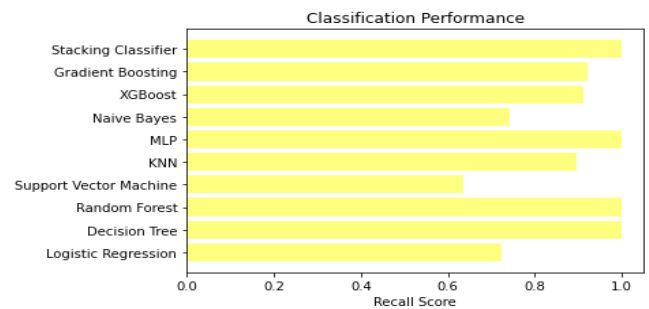
Fig 14 Recall graph
