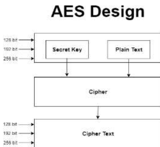
how it converts simple text into Cipher Text
