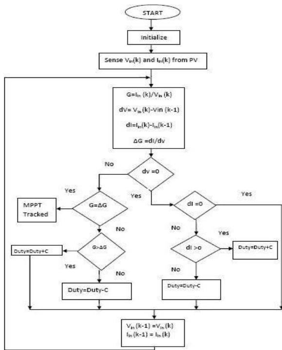
Figure. 6 Flowchart of the IC method.
